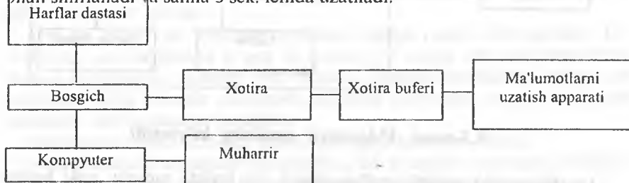
6.4-rasm. Teletekst tizimining tuzilishi
